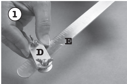
Loosen both wing nuts on part D and slide it onto the shaft of part E.
