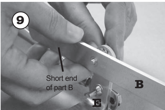
Slide part B onto the screw so that it rests on top of the locking washer. The shortest end part B should be parallel to the cutter handle.
