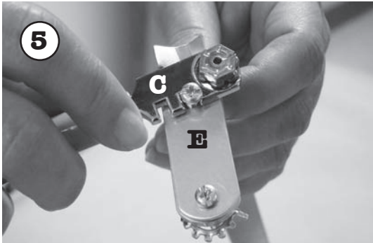
Slide cutter underneath screw head into the slot closest to the cutting head.
