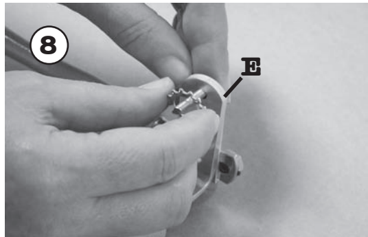
Slide the locking washer onto the screw with the teeth facing down.
