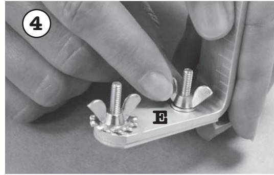
Loosen the wing nuts at the base of part E.
